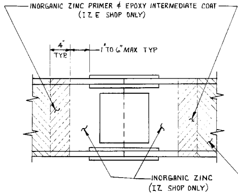
FIGURE - 1 @ BOLTED SPLICE SHOP COATINGS
