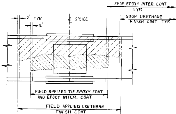
FIGURE - 2 @ BOLTED SPLICE FIELD COATINGS
